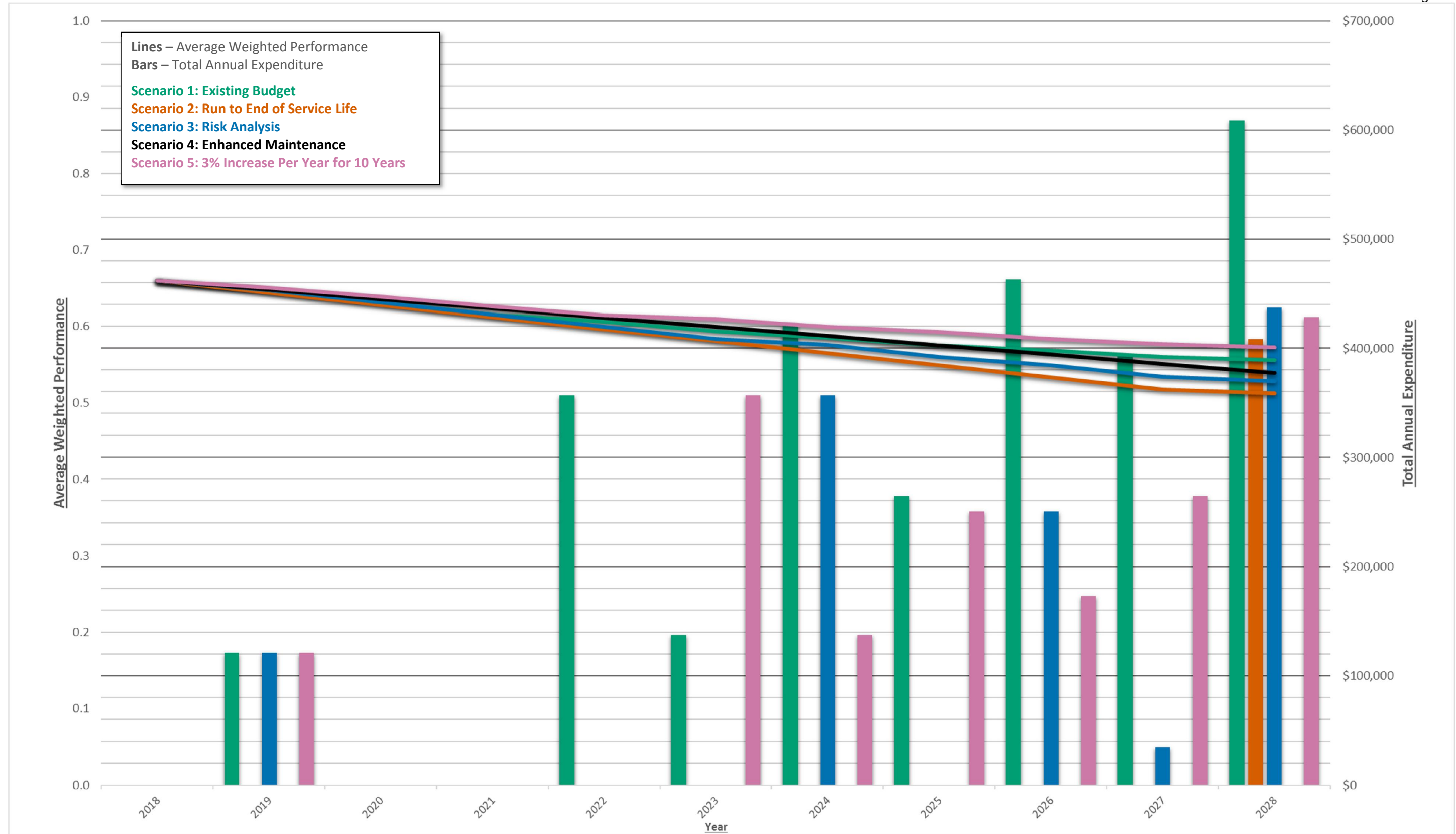
Figure 16: Expenditures and Performance of Bridge & Structure Assets
